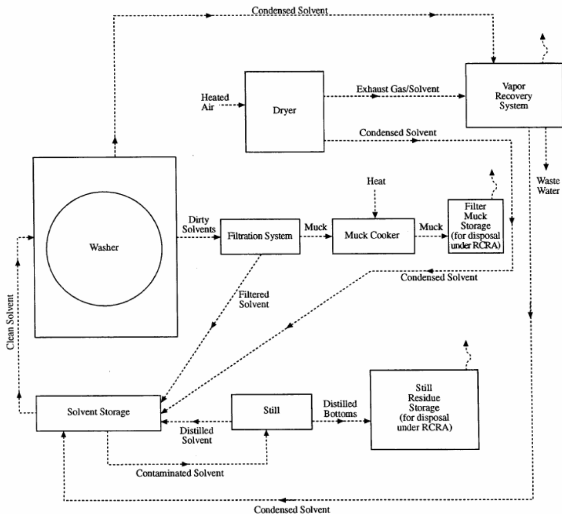
Figure 3 - Solvent Cycle in Dry Cleaning Operations
